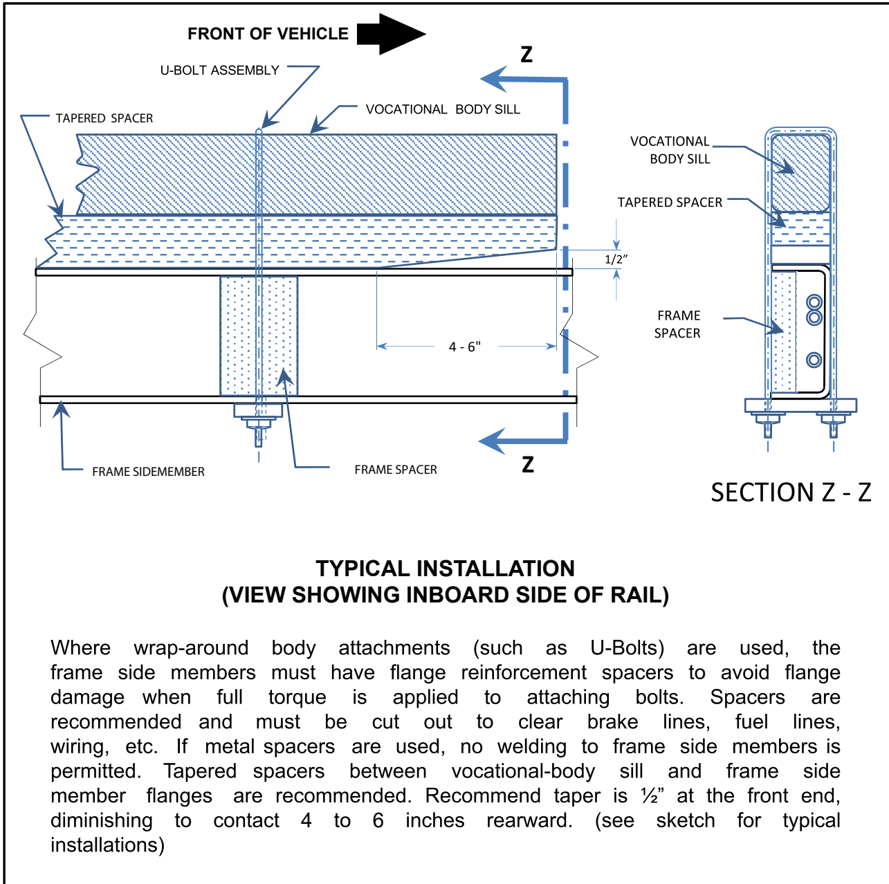
FIGURE C - CHASSIS CAB SUB-MOUNTINGSPACER
