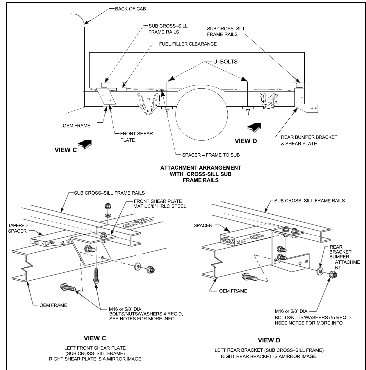
FIGURE B - TECHNIQUE #2 Shear Plates w/Cross-Frame
