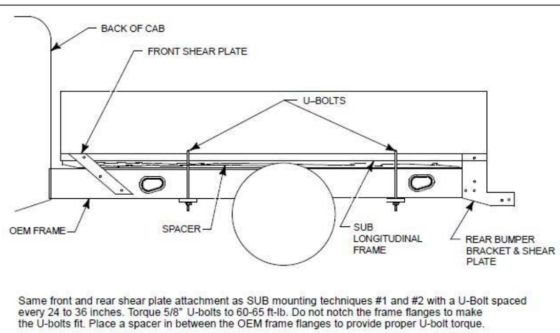
Figure E SUPER DUTY F-SERIES SUB MOUNTING FOR 60", 84", 108" AND 120" CA CHASSIS CABS
