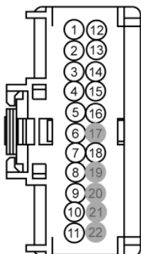
Male Connector (on blunt-cut pigtail)
