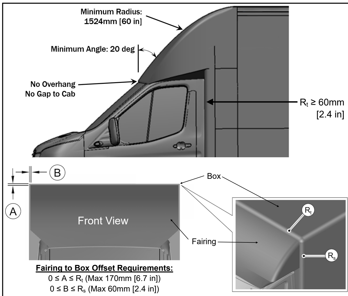
FIGURE 9 – SECOND UNIT BODY GEOMETRY RESTRICTIONS REQUIRED TO REALIZE ENHANCED FRONTAL AREA LIMITATION 2 MAXIMUM VALUES
