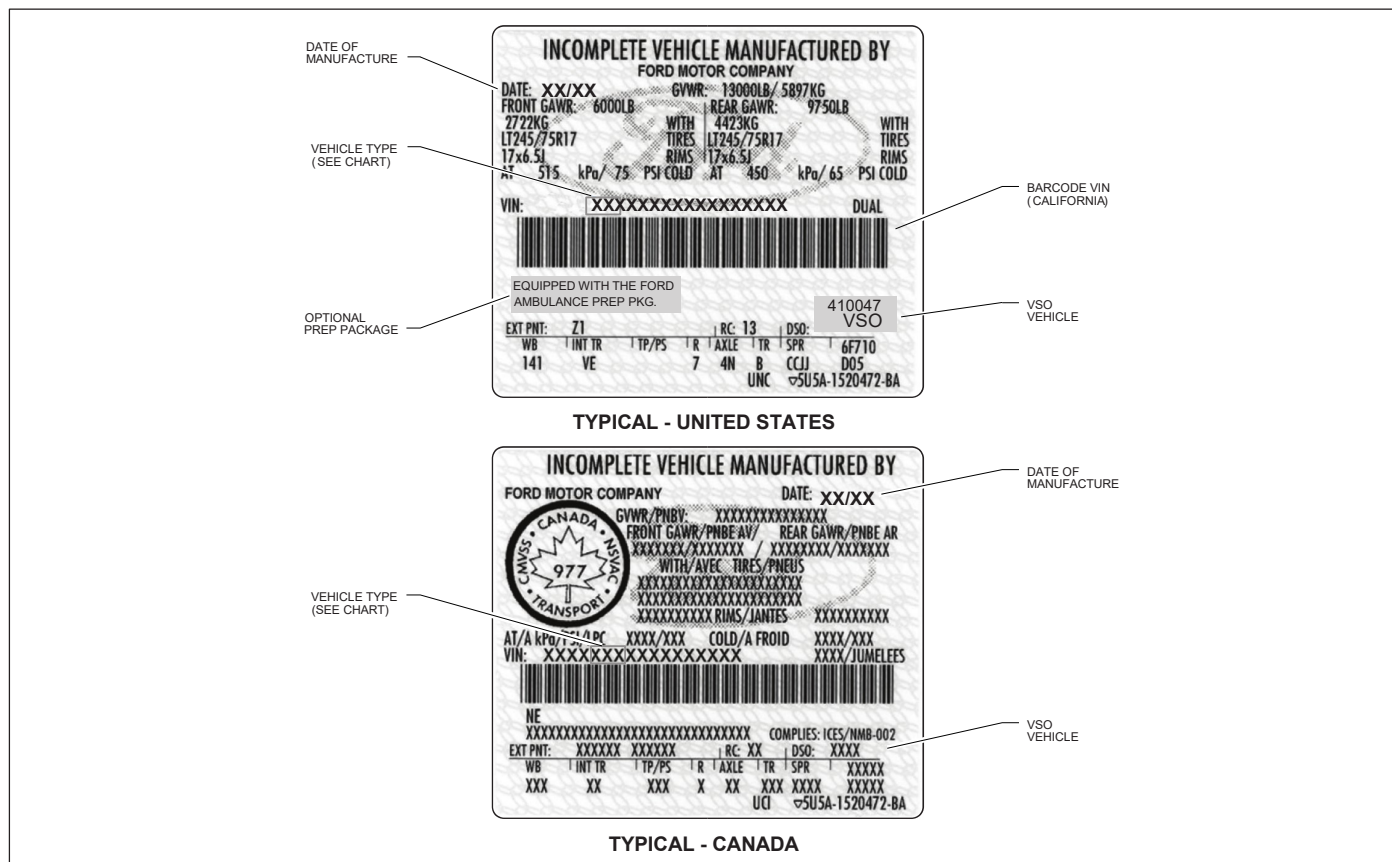
FIGURE 1 - SAMPLE INCOMPLETE VEHICLE INFORMATION LABELS
