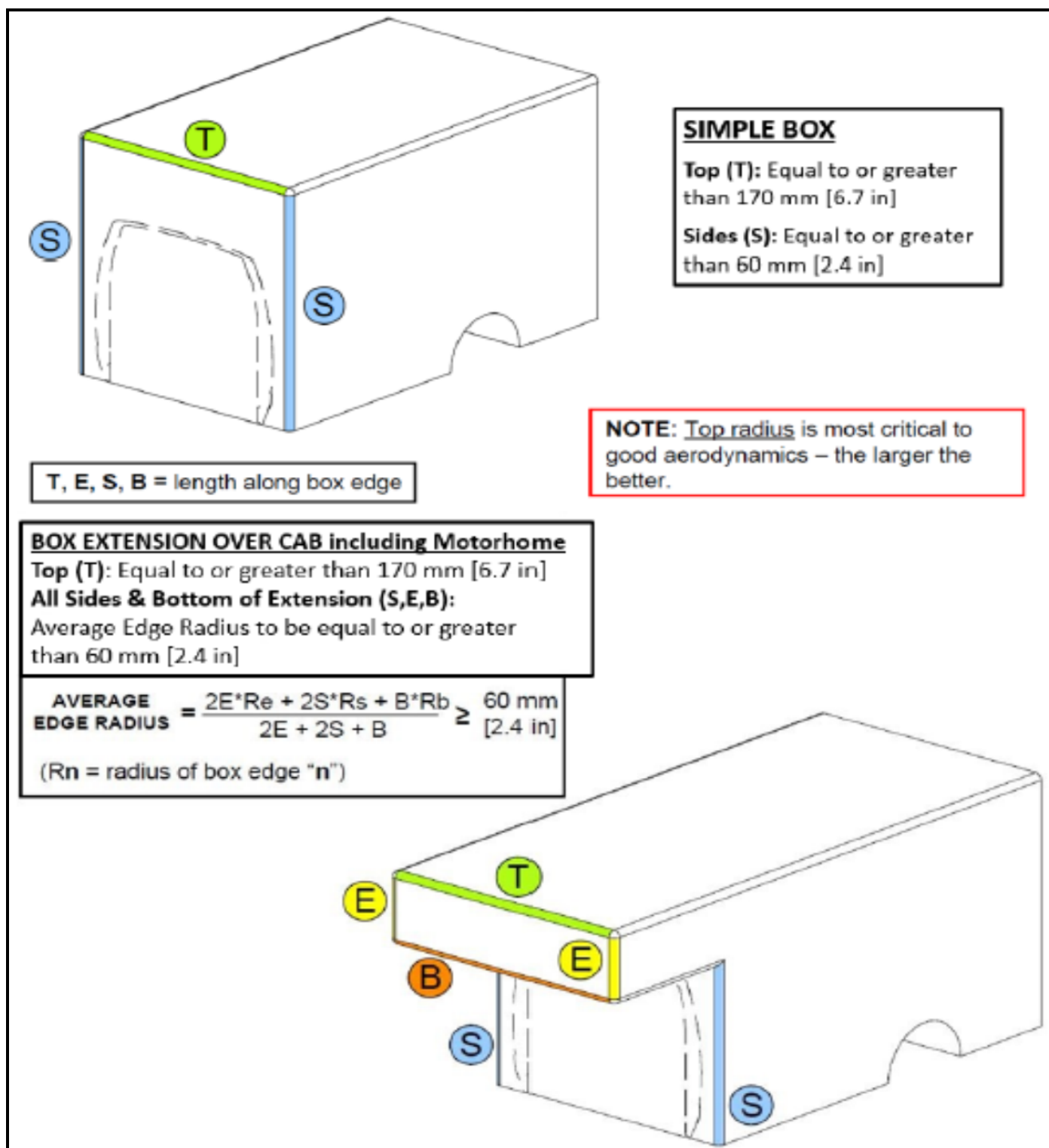
FIGURE 8 – SECOND UNIT BODY RADII RESTRICTIONS REQUIRED TO REALIZE ENHANCED FRONTAL AREA LIMITATION 1 MAXIMUM VALUES
