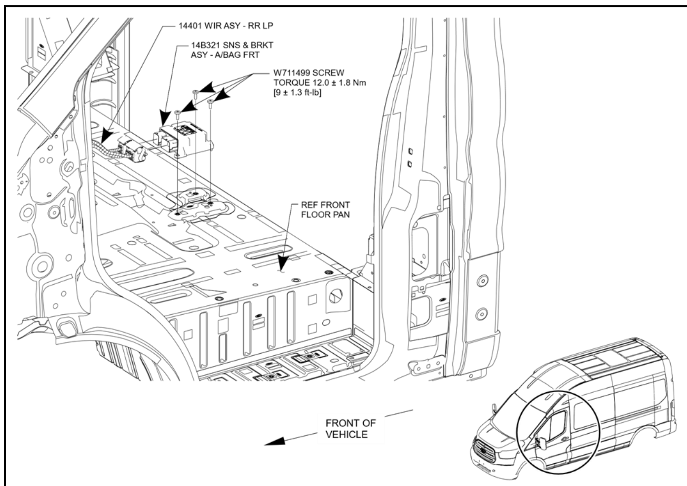
FIGURE 3C - TRANSIT RESTRAINT CONTROL MODULE MOUNTING
