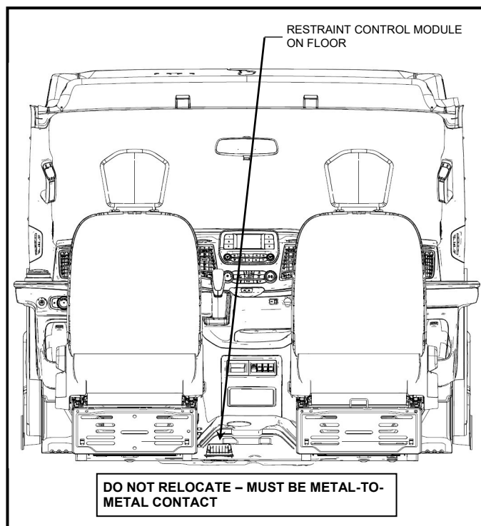
FIGURE 3B - TRANSIT RESTRAINT CONTROL MODULE
