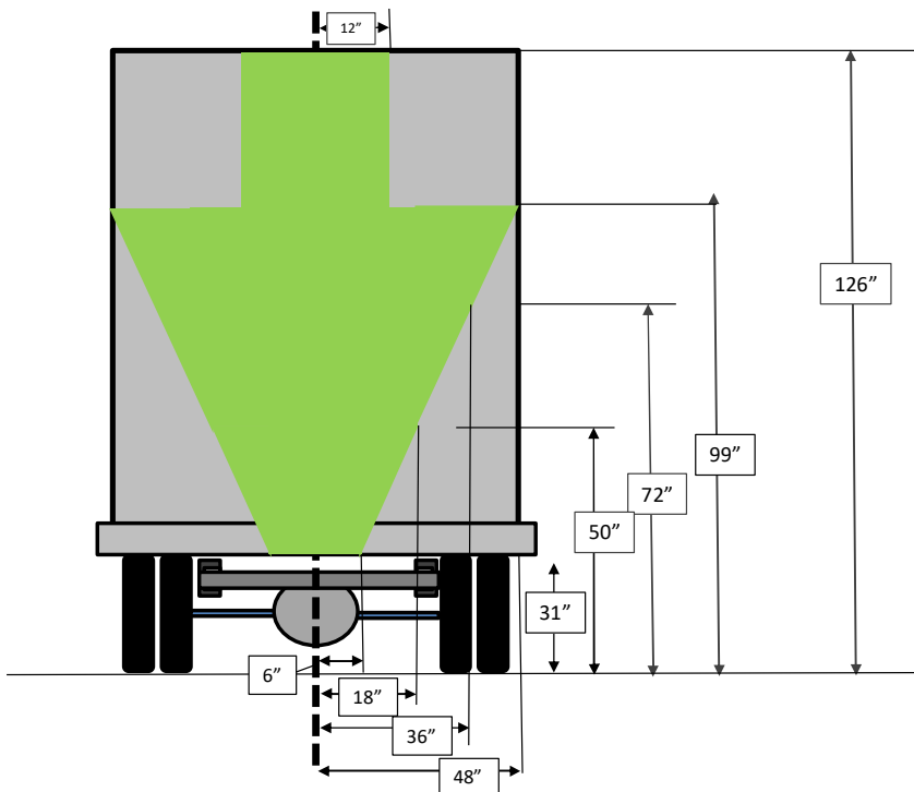
Figure 5: Coverage with 4.2 and 8 inch display, as shown at the rear plane of the vehicle
