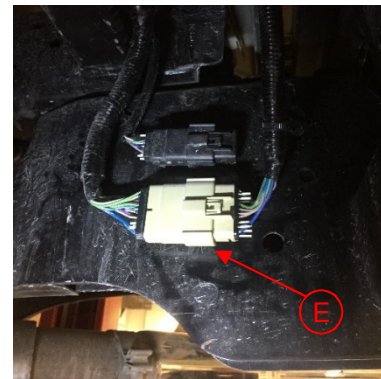
Figure 2: Box delete harness installation – jumper harness shown installed
