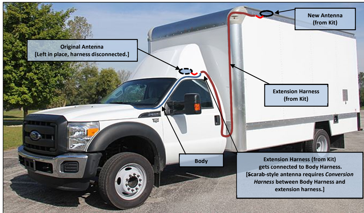
Figure 1: Example of antenna relocation kit installation
