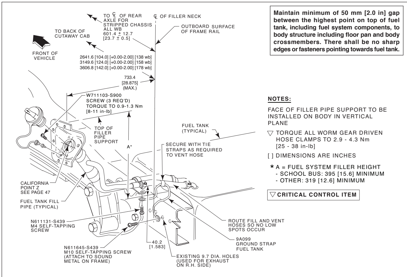
FIGURE J – E-350/450 CUTAWAY AND BASIC (STRIPPED) CHASSIS FUEL FILLER PIPE INSTALLATION FOR AFT-OF-AXLE FUEL TANK
