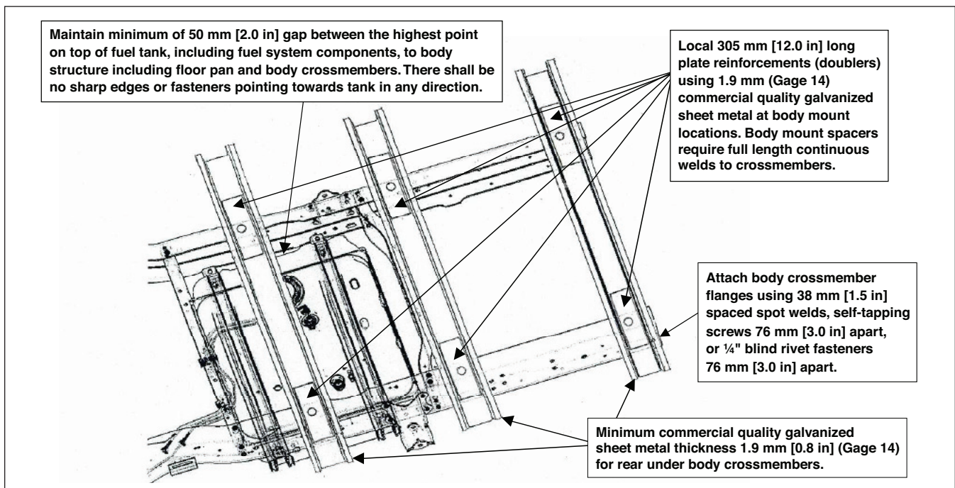
FIGURE I – E-350 SRW CUTAWAY WITH SCHOOL BUS PREPARATION PACKAGE
