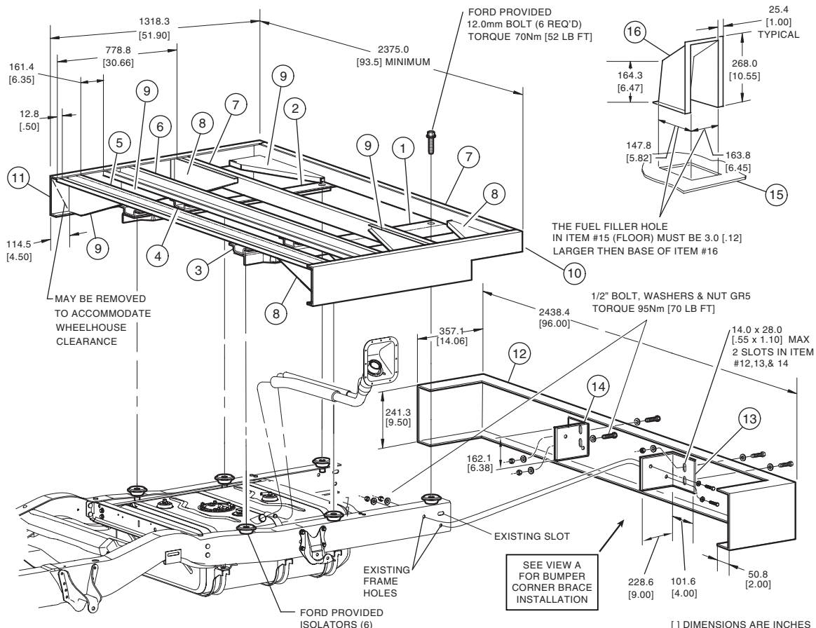
FIGURE K1 – E-SERIES DRW SCHOOL BUS FUEL SYSTEM AND FLOOR STRUCTURE
