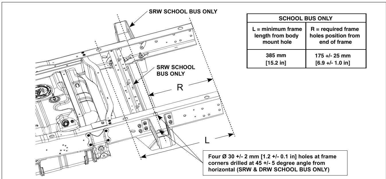
FIGURE H1 – E-350 CUTAWAY WITH SCHOOL BUS PREPARATION PACKAGE
