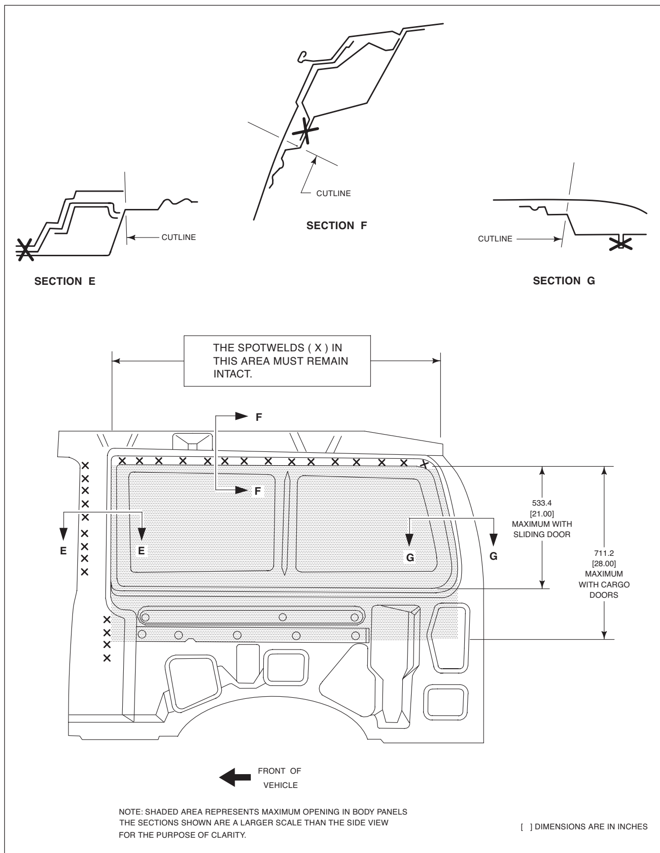
FIGURE F2 – BODY PANEL WINDOW REMOVAL AREA – E-SERIES (PASSENGER SIDE – R.H.)
