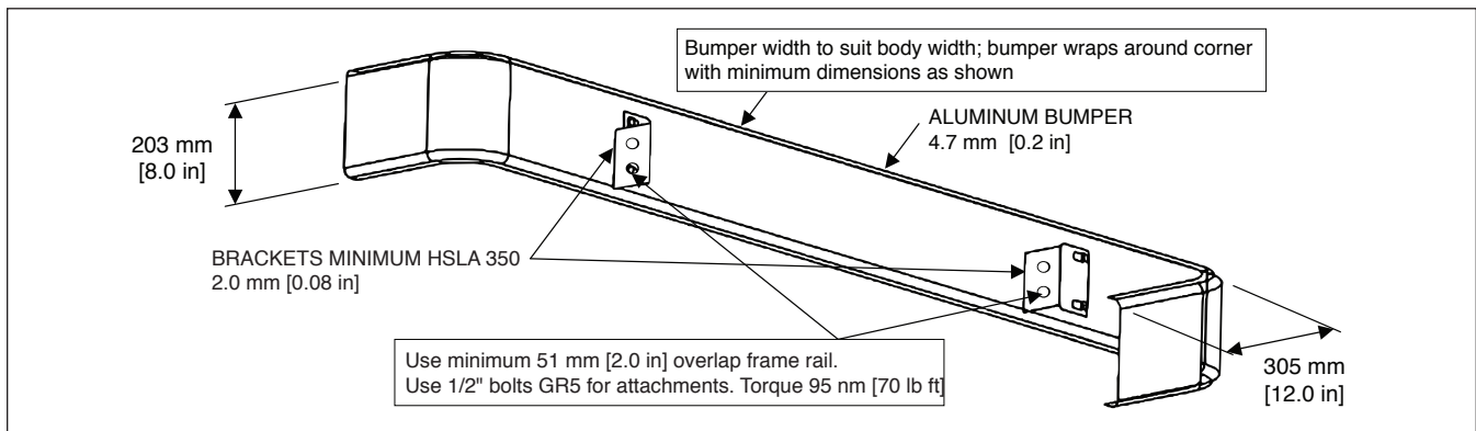
FIGURE H2 – E-350 SRW CUTAWAY WITH SCHOOL BUS PREPARATION PACKAGE
