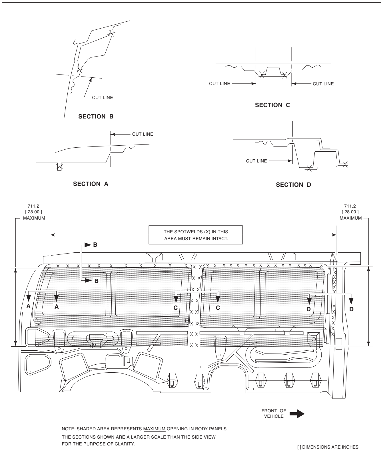
FIGURE F1 – BODY PANEL WINDOW REMOVAL AREA – E-SERIES (DRIVER SIDE – L.H.)
