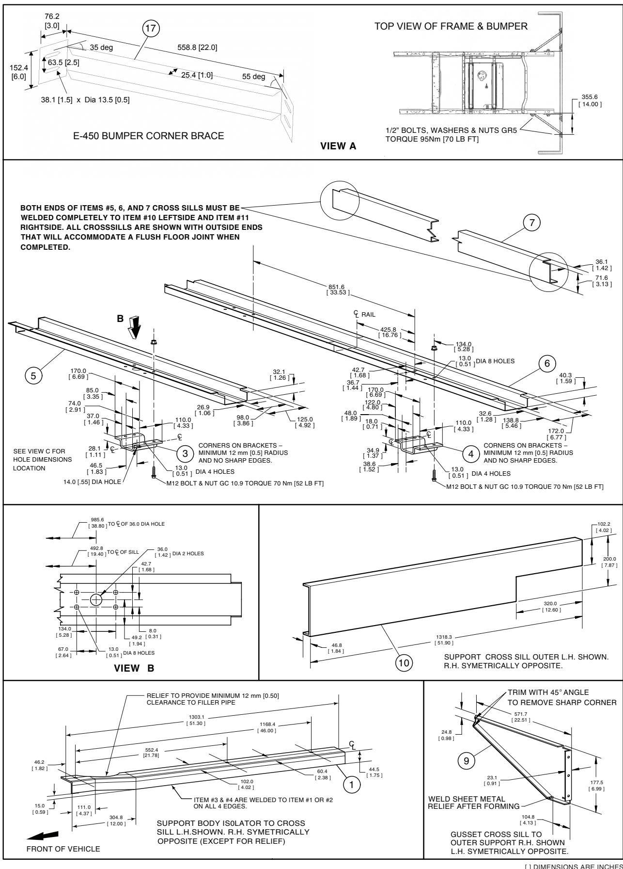
FIGURE K2 – E-SERIES SCHOOL BUS FUEL SYSTEM AND FLOOR STRUCTURE (OVER 4536 KG [10,000 LB] GVWR)
