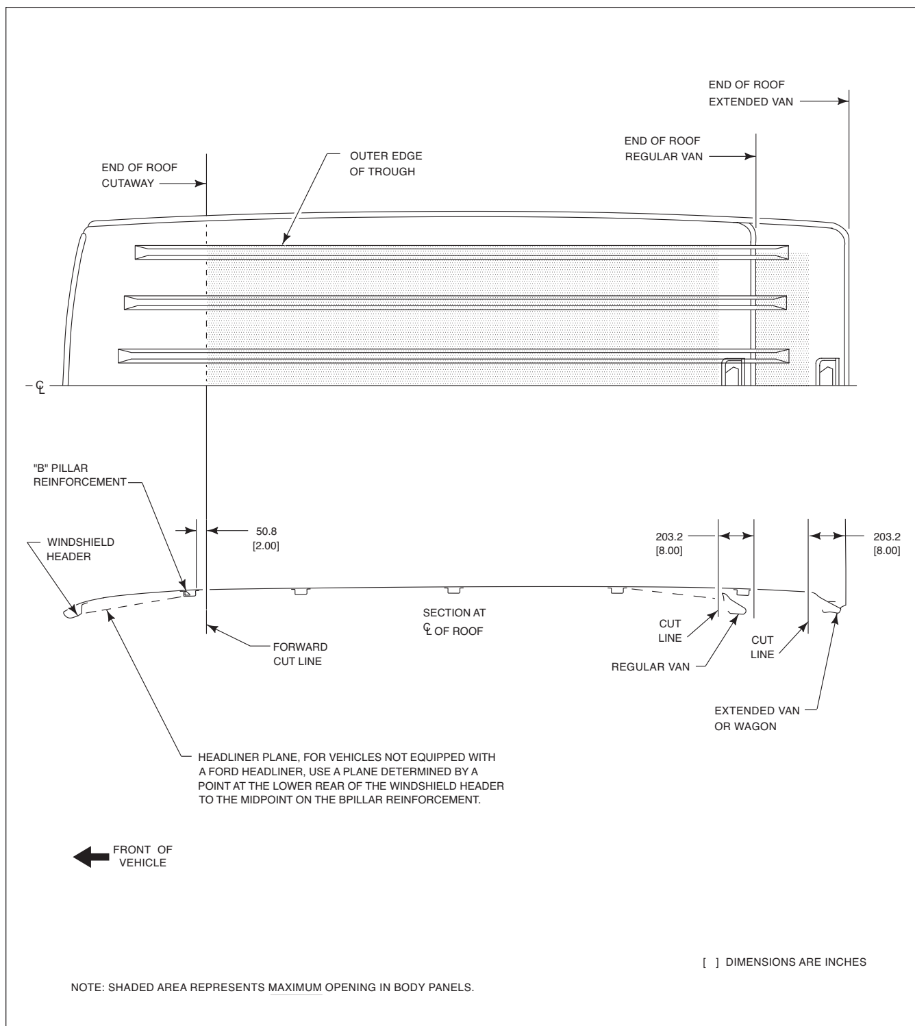
FIGURE F3 – ROOF PANEL REMOVAL AREA – E-SERIES
