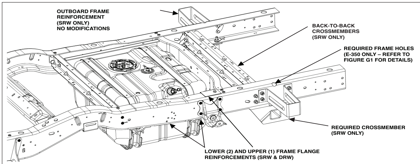
FIGURE G1 – E-SERIES CUTAWAY WITH SCHOOL BUS PREPARATION PACKAGE
