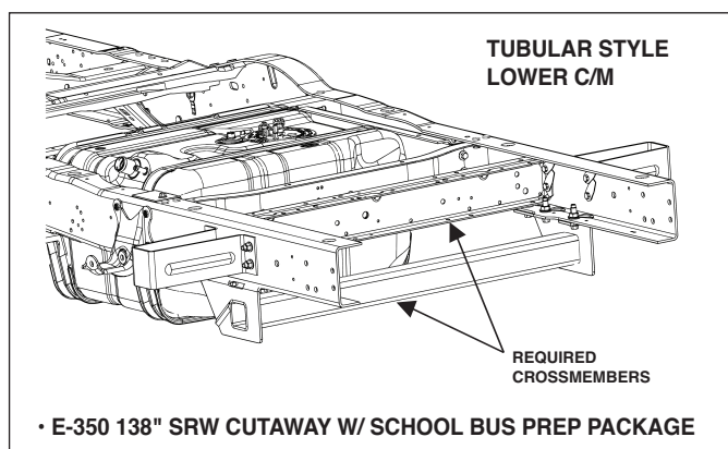
FIGURE G2 – E-350 CUTAWAY REQUIRED REAR CROSSMEMBER FOR SRW SCHOOL BUS PREPARATION PACKAGE
