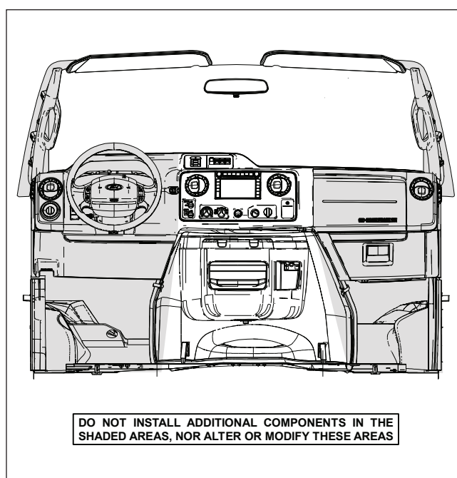
FIGURE D – E-SERIES OCCUPANT PROTECTION ZONE
