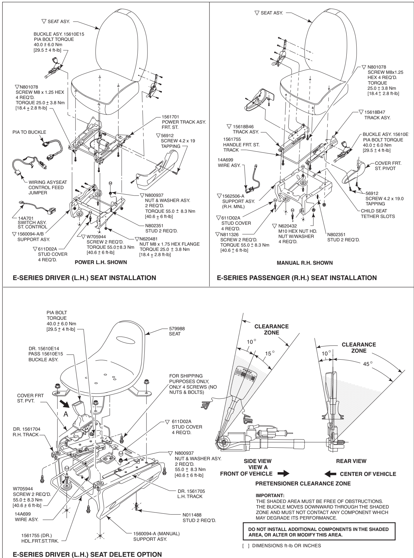
FIGURE B – E-SERIES FRONT SEAT INSTALLATION
